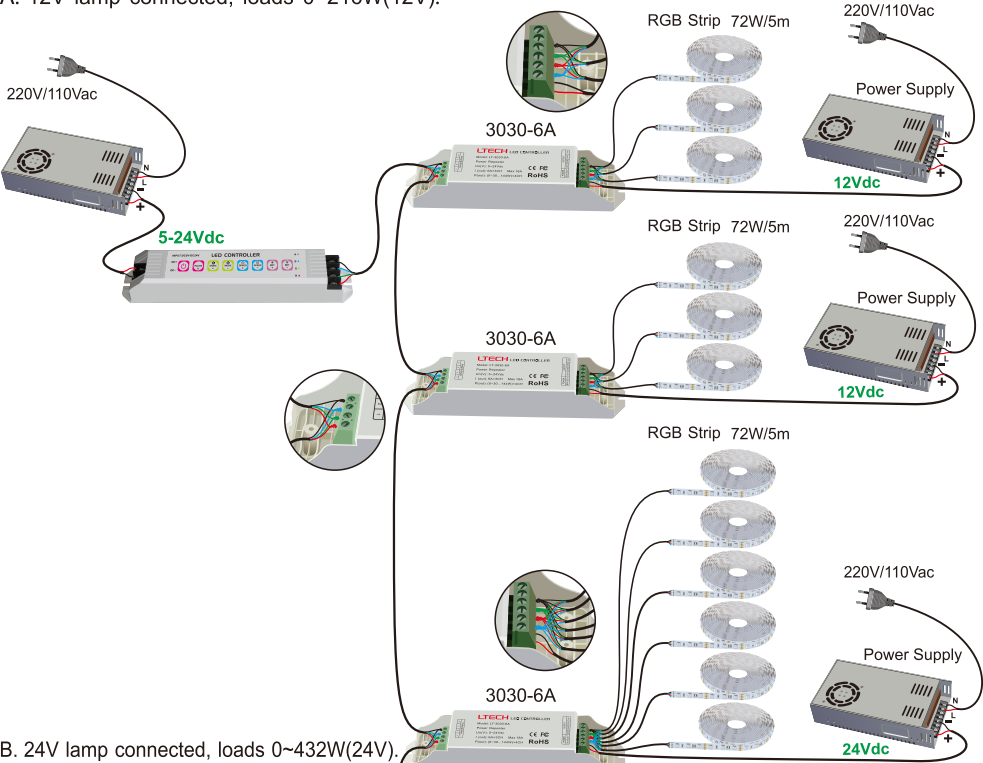
B. 24V lamp connected, loads 0~432W(24V).
